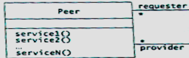
Figure 6-19 Peer-to-peer architectural style (UML class diagram). Peers can request services from and provide services to other peers.
