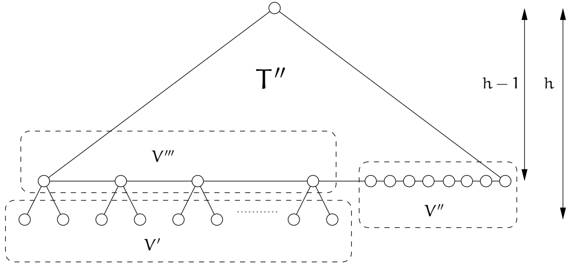
Figure 4.2: The heap in Problem 90.
