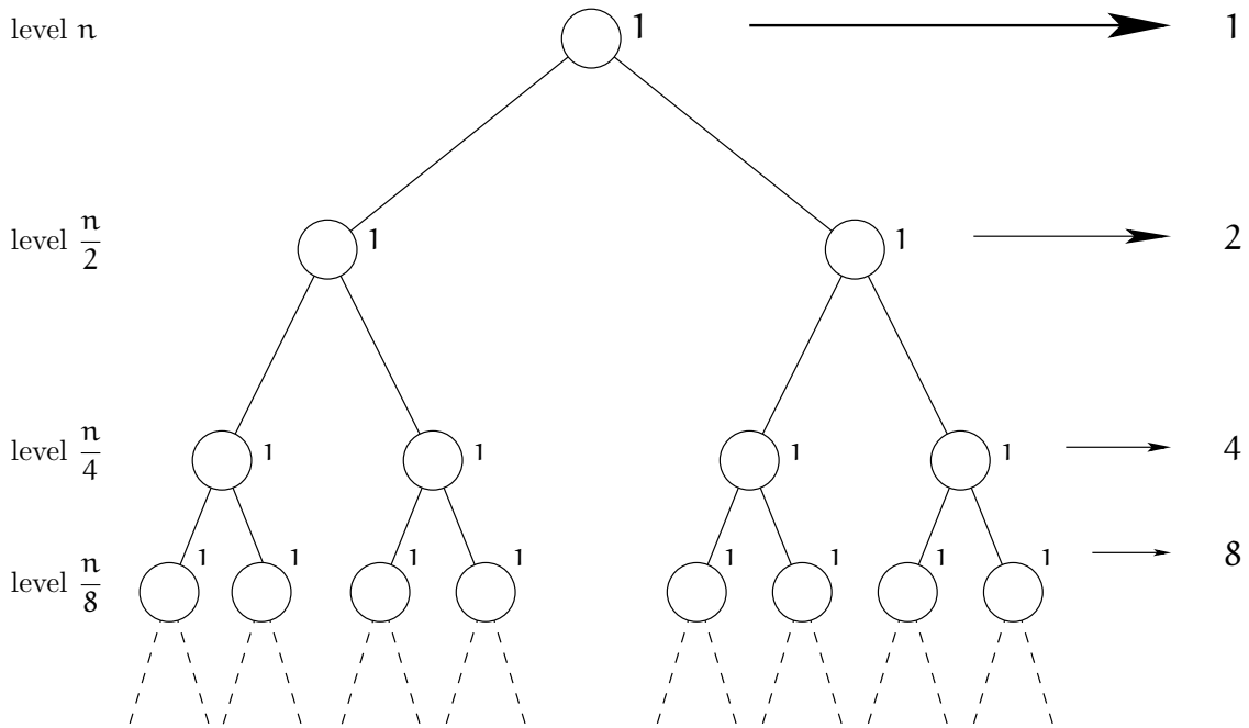
Figure 3.5: The recursion tree of T(n) = 2T\left(\frac{n}{2}\right) + 1 .
