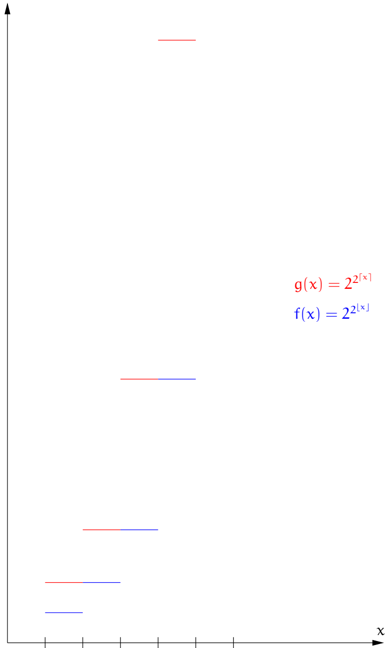
Figure 1.1: f(x) and g(x) from Problem 30.
