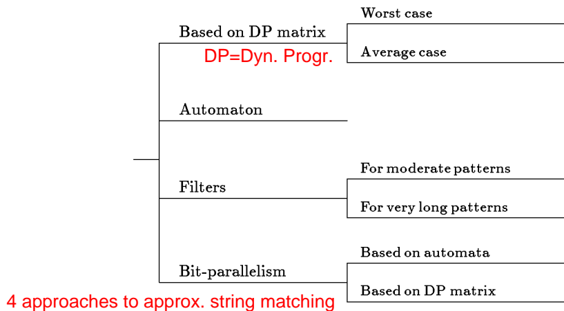
Fig. 4. Taxonomy of the types of solutions for online searching.
