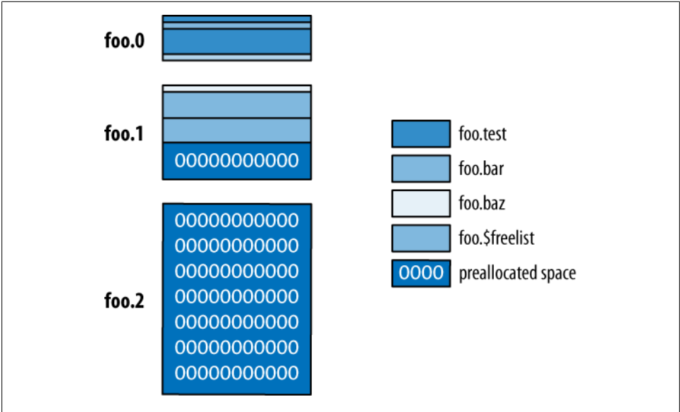
Figure C-1. Namespaces and extents
