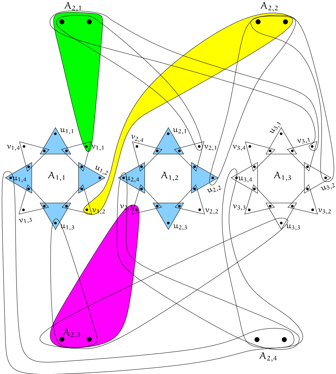
Figure 7.9: The reduction 3SAT \propto 3DM . The CNF is Q = (x_1 \vee x_2 \vee x_3) (x_1 \vee \overline{x_2} \vee \overline{x_3}) (\overline{x_1} \vee x_2 \vee \overline{x_3}) (\overline{x_1} \vee \overline{x_2} \vee \overline{x_3}) . We put (v_{2,3}, s_{1,3}, s_{2,3}) in the matching (in magenta). That forces the addition of the blue triples from A_{1,2} to the matching.
