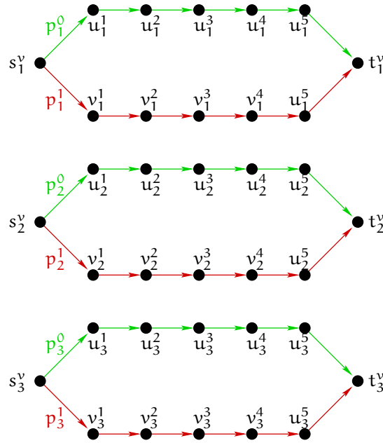
Figure 7.18: The reduction 3\text{SAT} \times \text{EDP} : the first stage of the construction.
