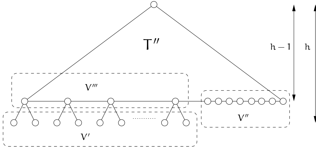
Figure 8.2: The heap in Problem 152.
