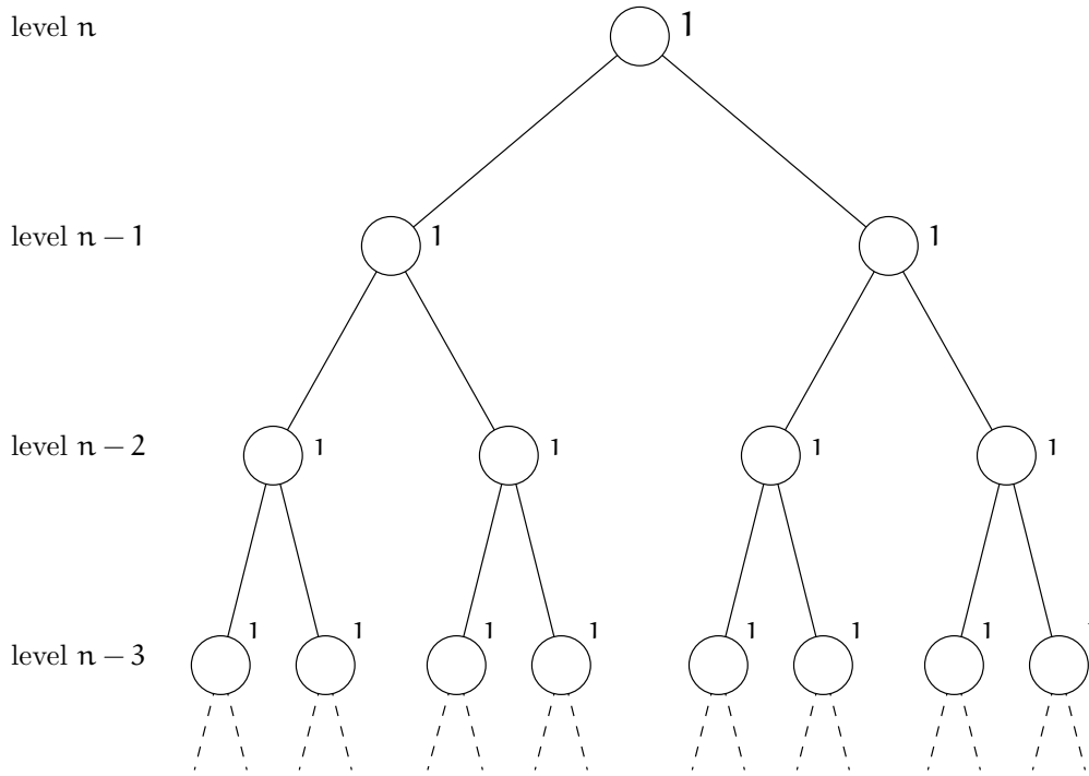
Figure 3.2: The recursion tree of T(n) = 2T(n-1) + 1 .
