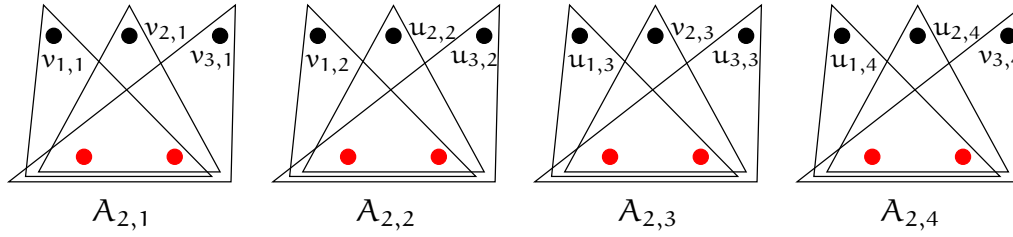
Figure 7.3: The four crowns in the construction for Q = (x_1 \vee x_2 \vee x_3)(x_1 \vee \bar{x}_2 \vee \bar{x}_3)(\bar{x}_1 \vee x_2 \vee \bar{x}_3)(\bar{x}_1 \vee \bar{x}_2 \vee x_3) . A_{2,1} corresponds to clause q_1 and so on. The red dots represent the common anonymous elements.
