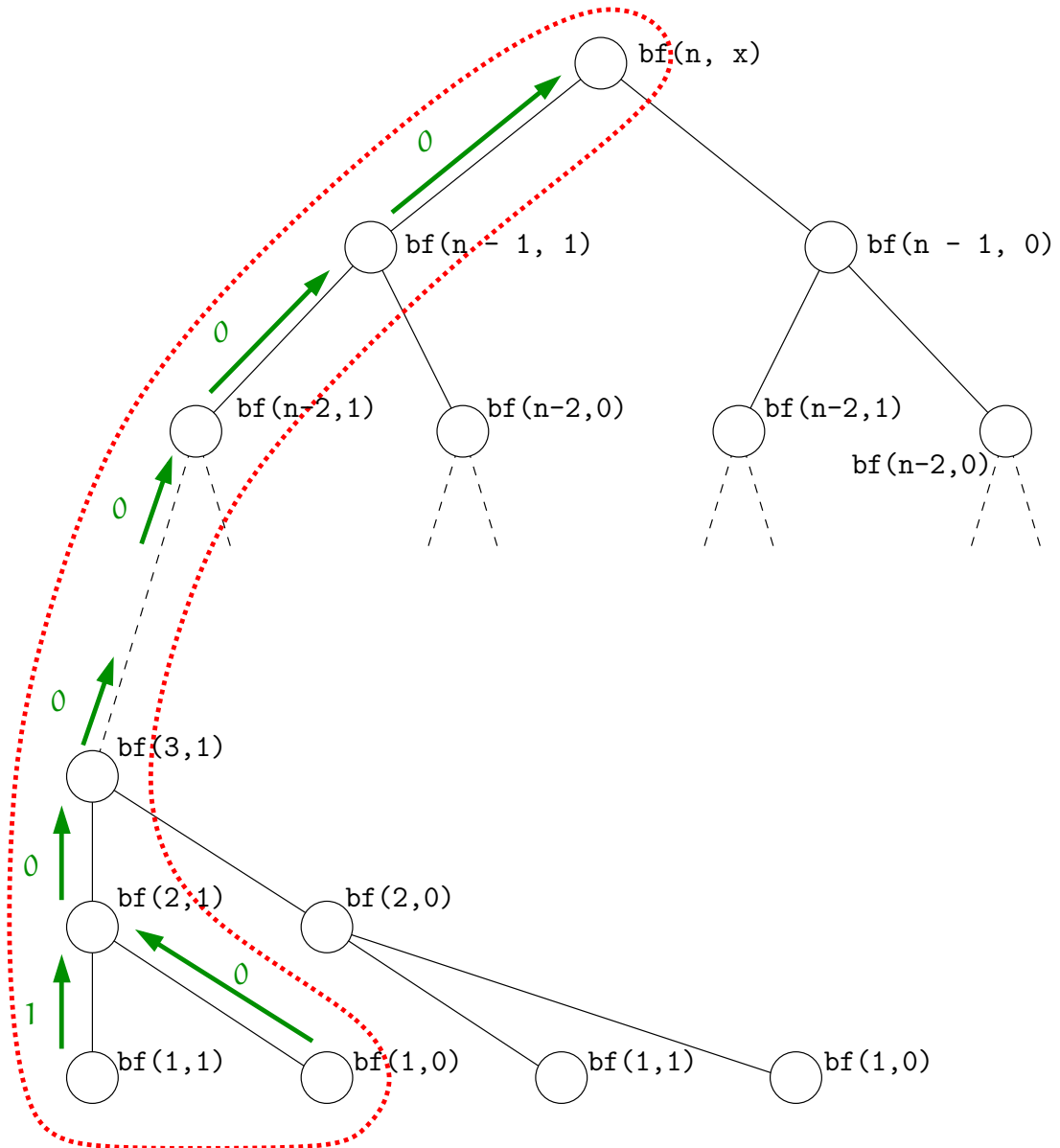
Figure 6.1: The recursion tree of the fragment in Problem 122. We draw the whole tree, i.e. what the tree would be if the considerations about the && operator were not taken into account. The part of the tree that corresponds to the execution of the fragment when these considerations are taken into account, is outlined with dashed red line. The flow of the returned values is drawn in green.
